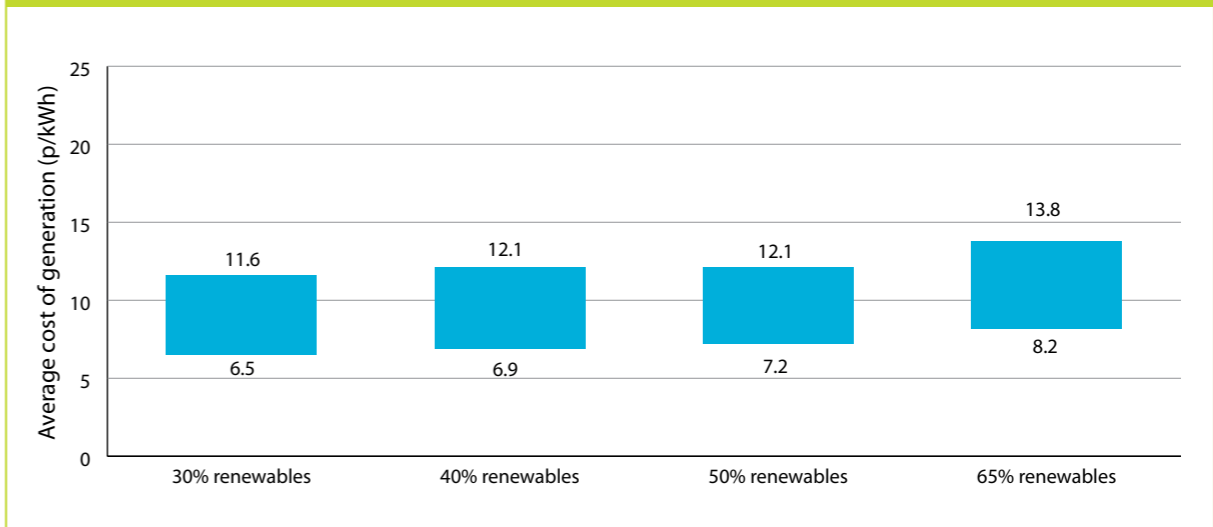
Figure 1.13: Range for average electricity generation costs in renewable generation scenarios (2030)
