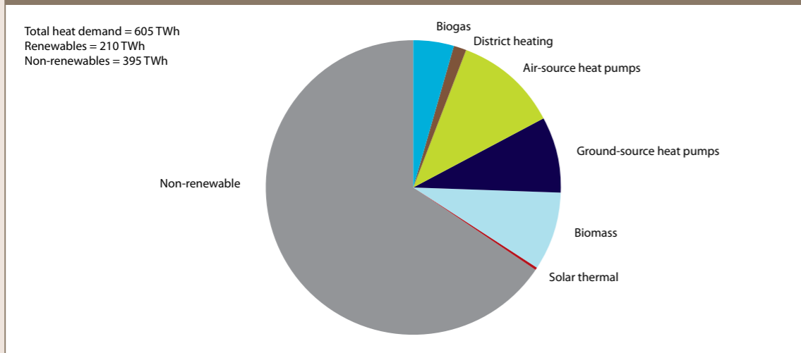
Figure B4: Fourth budget Medium abatement scenario: heat technologies (2030)
