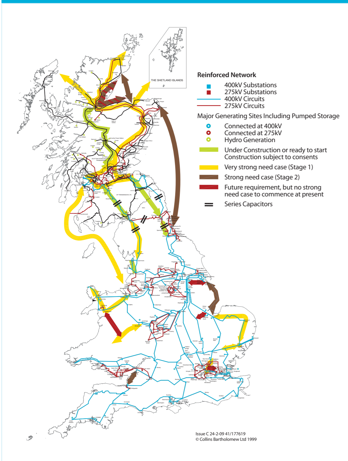
Figure B2.7: Map of ENSG reinforcements required to 2020
