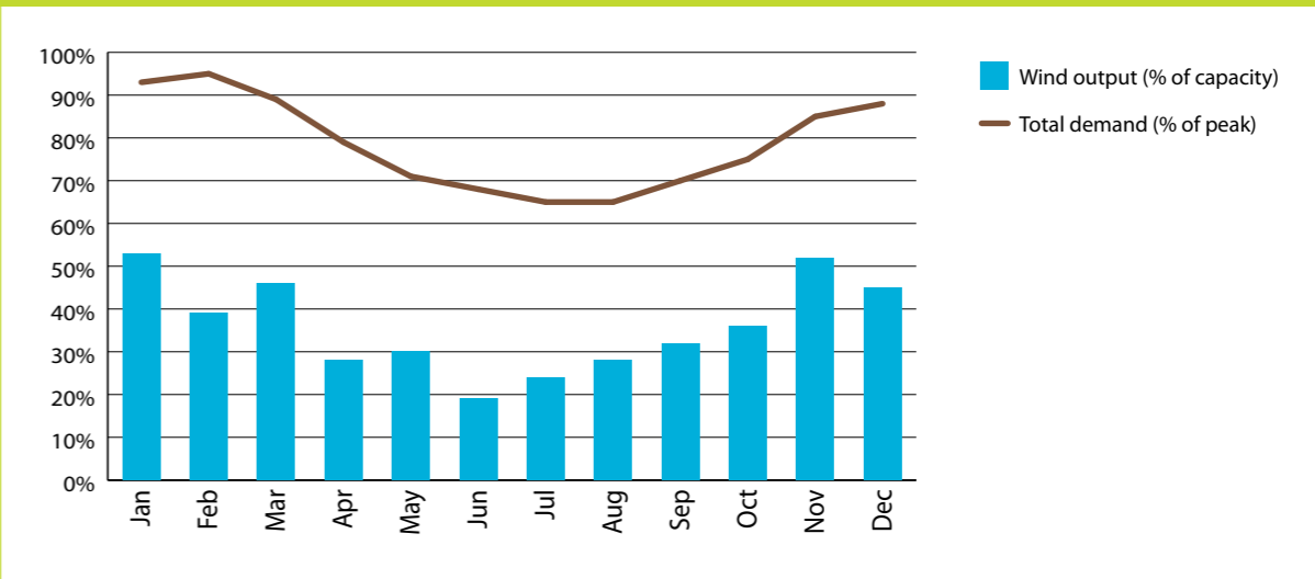
Figure 1.3: Seasonality of wind generation versus seasonality of demand
