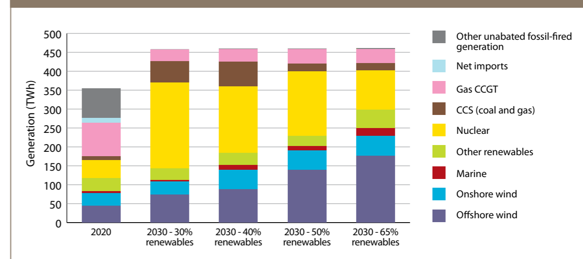
Figure 3: Renewable generation scenarios to 2030
