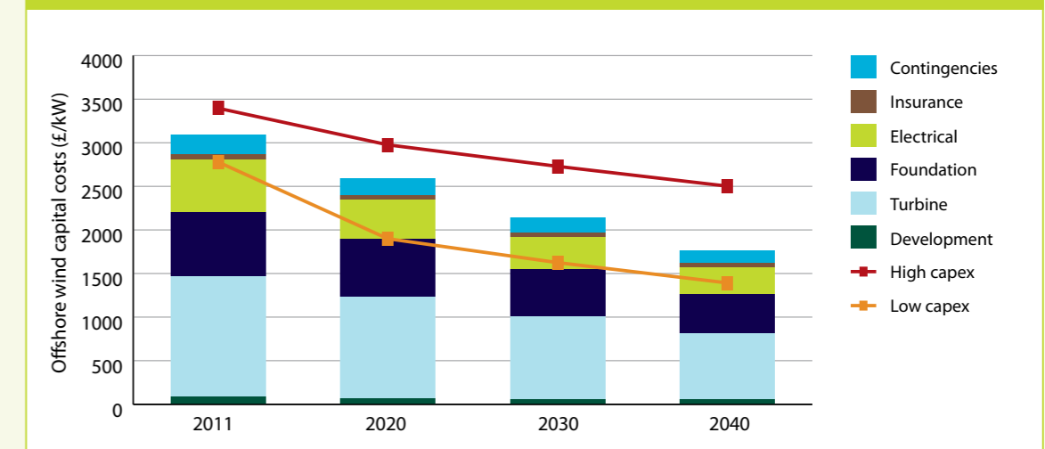
Figure B1.11: Projected offshore wind capital costs (2011, 2020, 2030, 2040)
