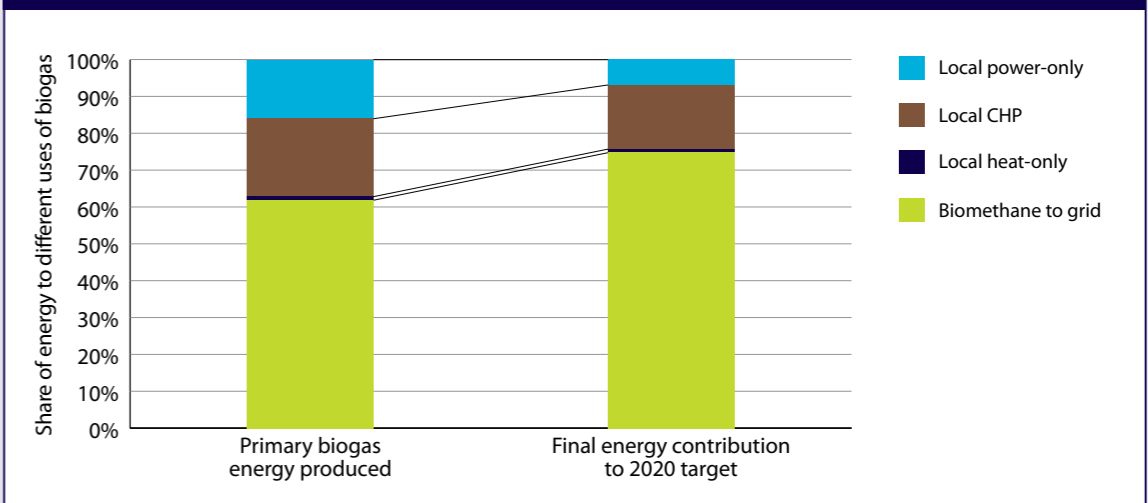
Figure B3.2a: Breakdown of primary and final biogas energy shares in SKM scenarios
